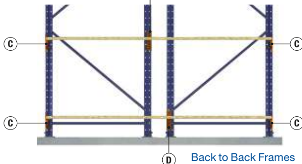
Frame and Post
