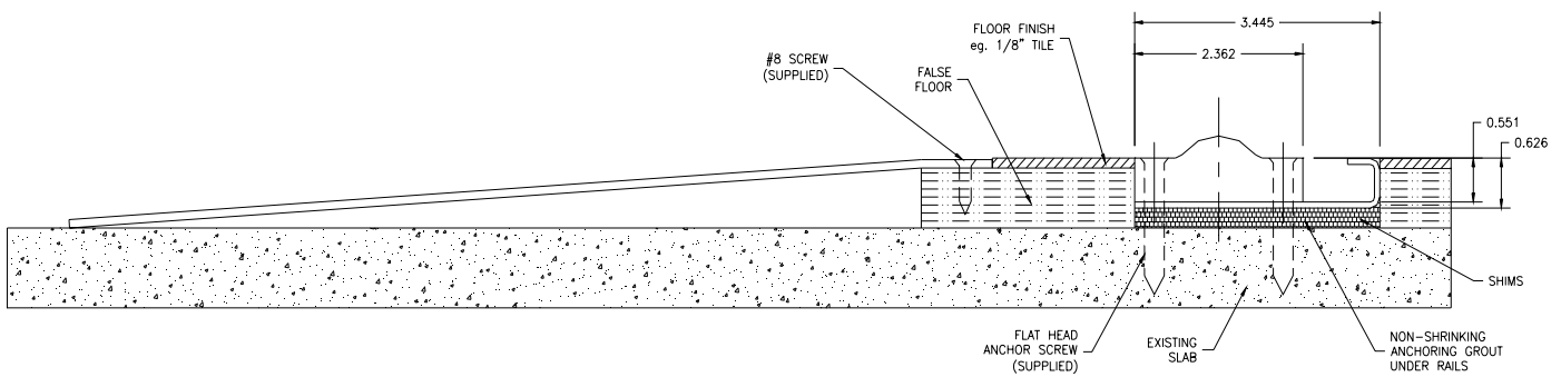
Figure 4 SECTION VIEW OF 12" ADA RAMP
