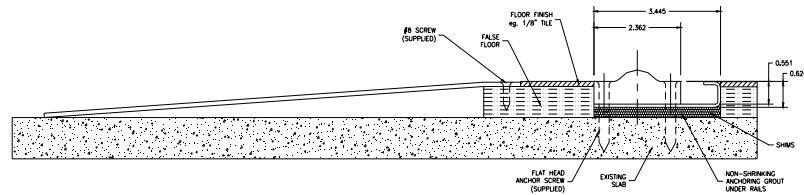
Figure 4 SECTION VIEW OF 12" ADA RAMP
