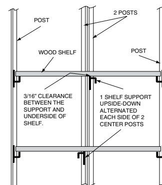
Depth (side) Section of Two Back-to-Back Units (with one chipboard shelf through both
